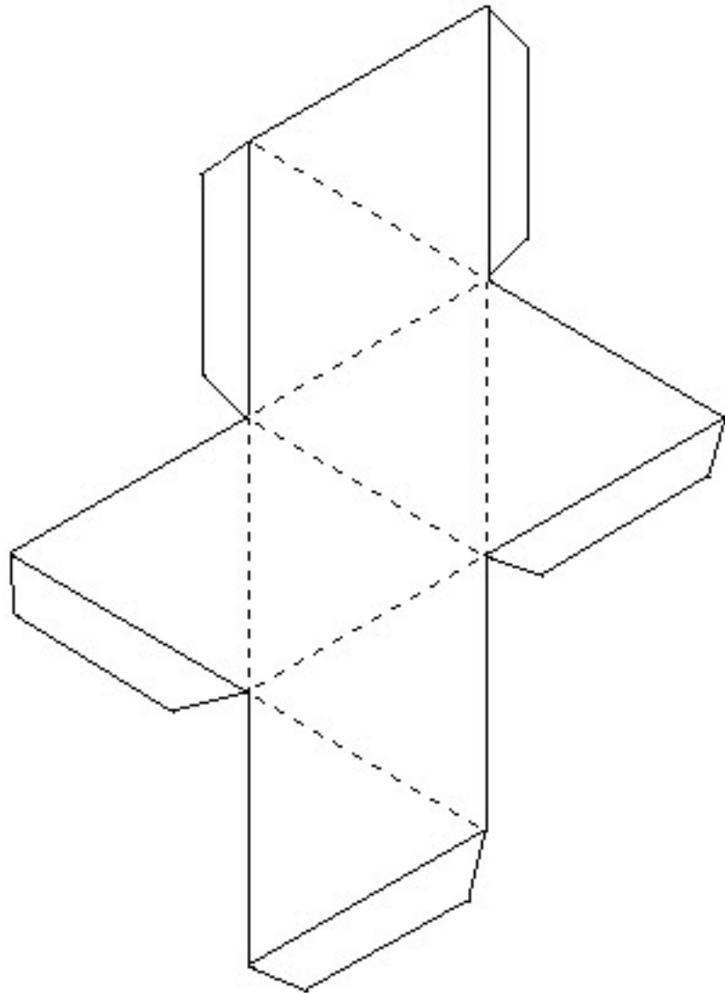
Net Octahedron
